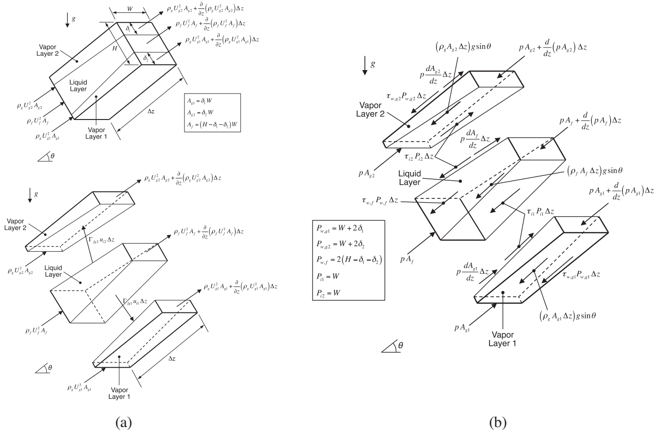
Fig. 8. (a) Momentum conservation applied to control volumes of length \Delta z for combined two-phase flow and for individual layers. (b) Force terms pertaining to control volumes of individual layers.
