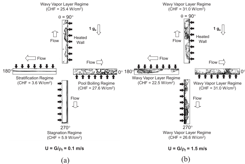
Fig. 1. Slightly subcooled ( \Delta T_{sub,0} = 3^\circ \text{C} ) flow boiling CHF regimes at 1 - g_e corresponding to different flow orientations for inlet liquid velocities (a) U = G/\rho_f = 0.1 \text{ m/s} and (b) U = G/\rho_f = 1.5 \text{ m/s} . CHF regime and magnitude are highly dependent on orientation for the lower velocity and independent of orientation for the higher velocity [37].
