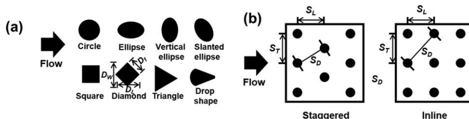
Fig. 2. Geometrical configurations of (a) pin fin shapes and (b) flow types.
