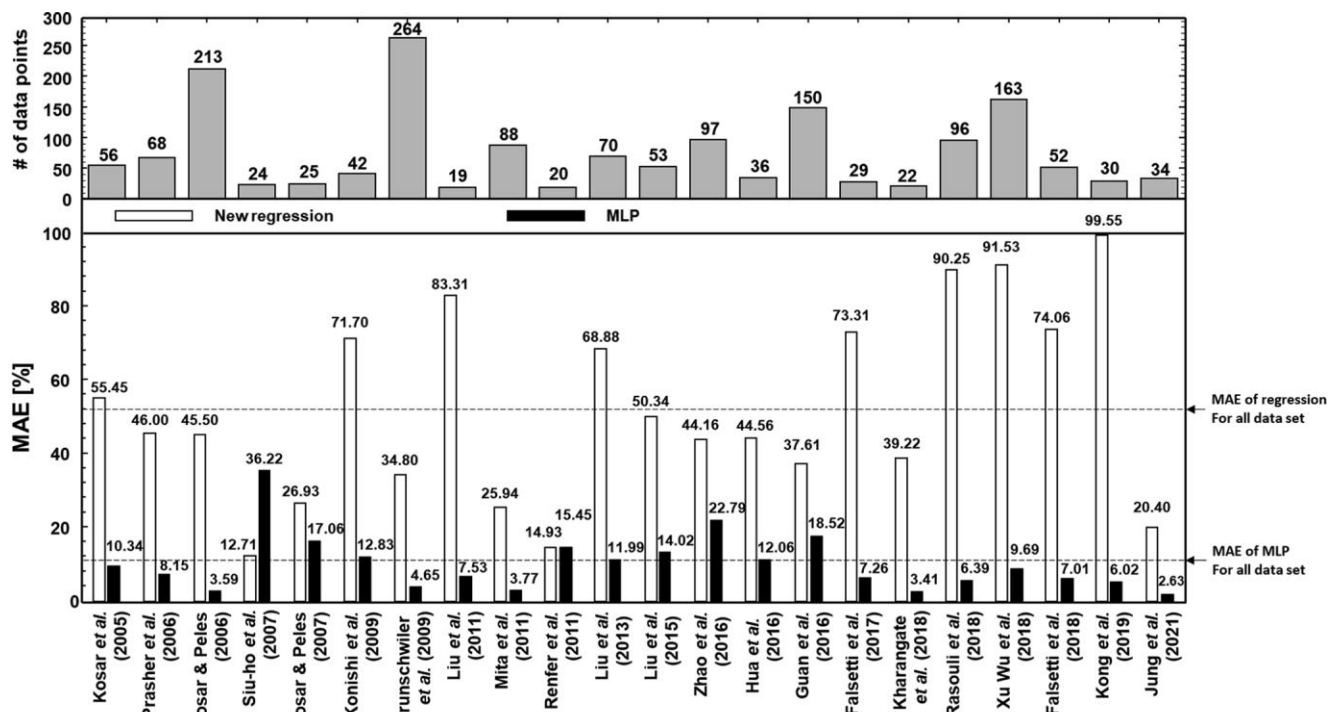
Fig. 14. Comparison of individual experimentally determined friction factor data points with MLP.
