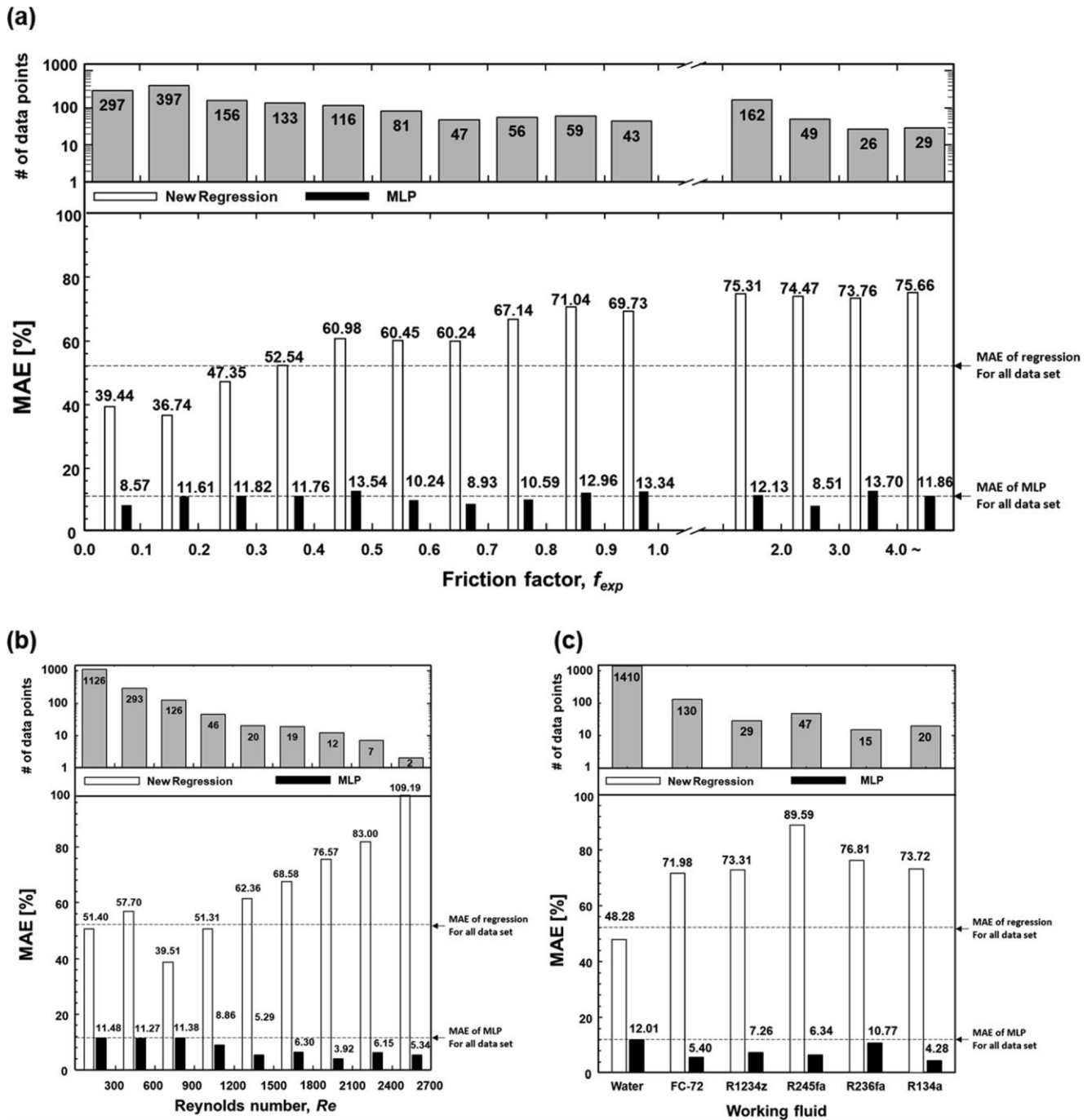
Fig. 12. Distribution of MAE in predictions of new regression correlation and MLP model according to operational conditions: (a) friction factor, (b) Reynolds number, and (c) working fluid.
