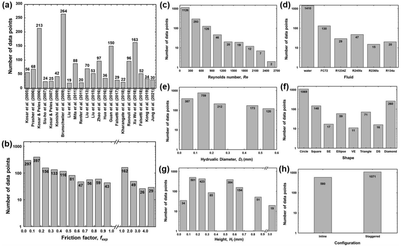
Fig. 3. Distribution of data points (a) sources, (b) friction factor, (c) Re , and (d) working fluids, and geometric parameters of (e) pin fin diameter, (f) pin fin shape, (g) pin fin height, and (h) fin configuration.
