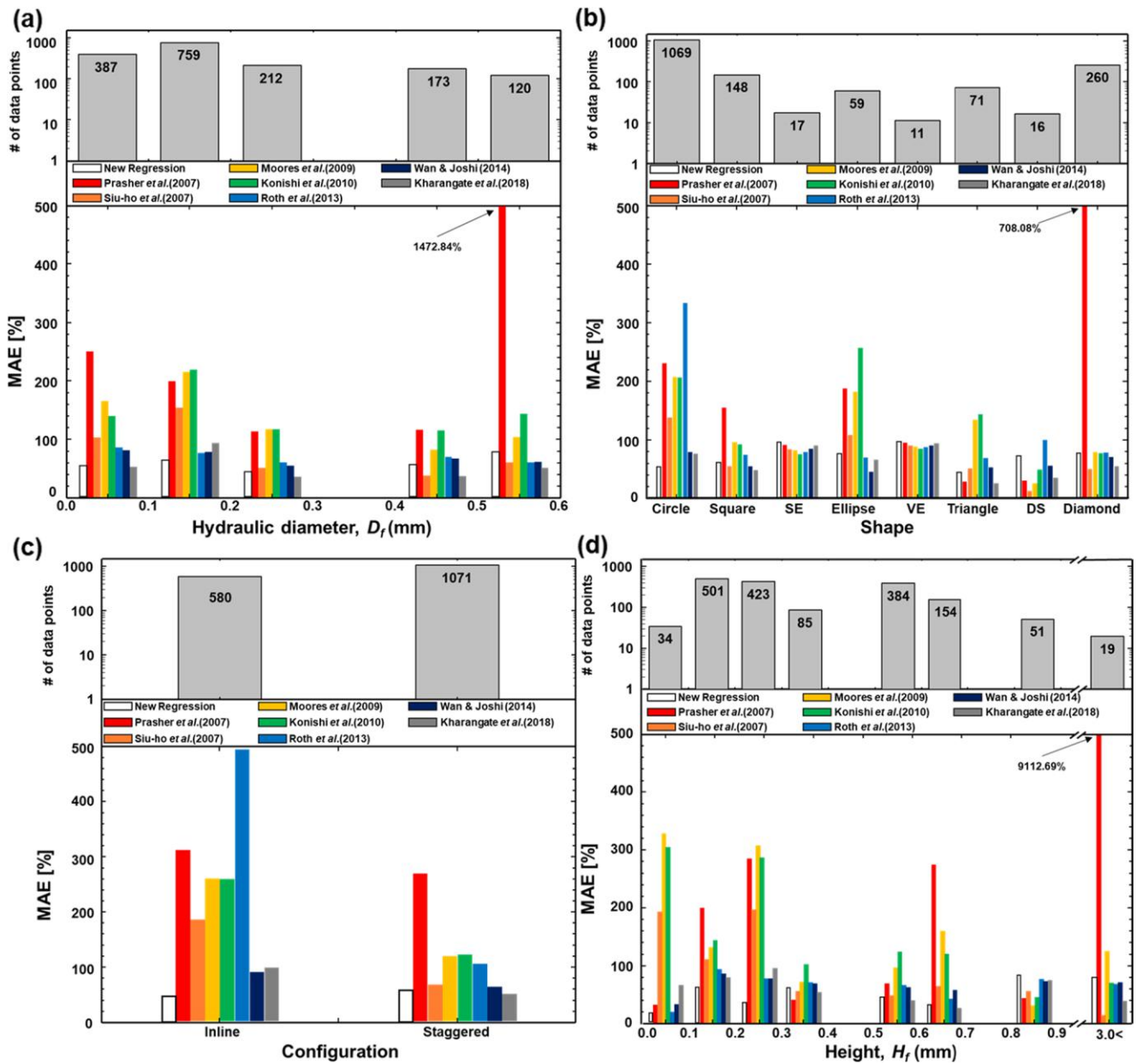
Fig. 10. Distribution of MAE in predictions of new regression correlation and previous correlations for data point relative geometrical conditions: (a) hydraulic diameter of pin fin, (b) fin shape, (c) fin configuration, and (d) fin height.
