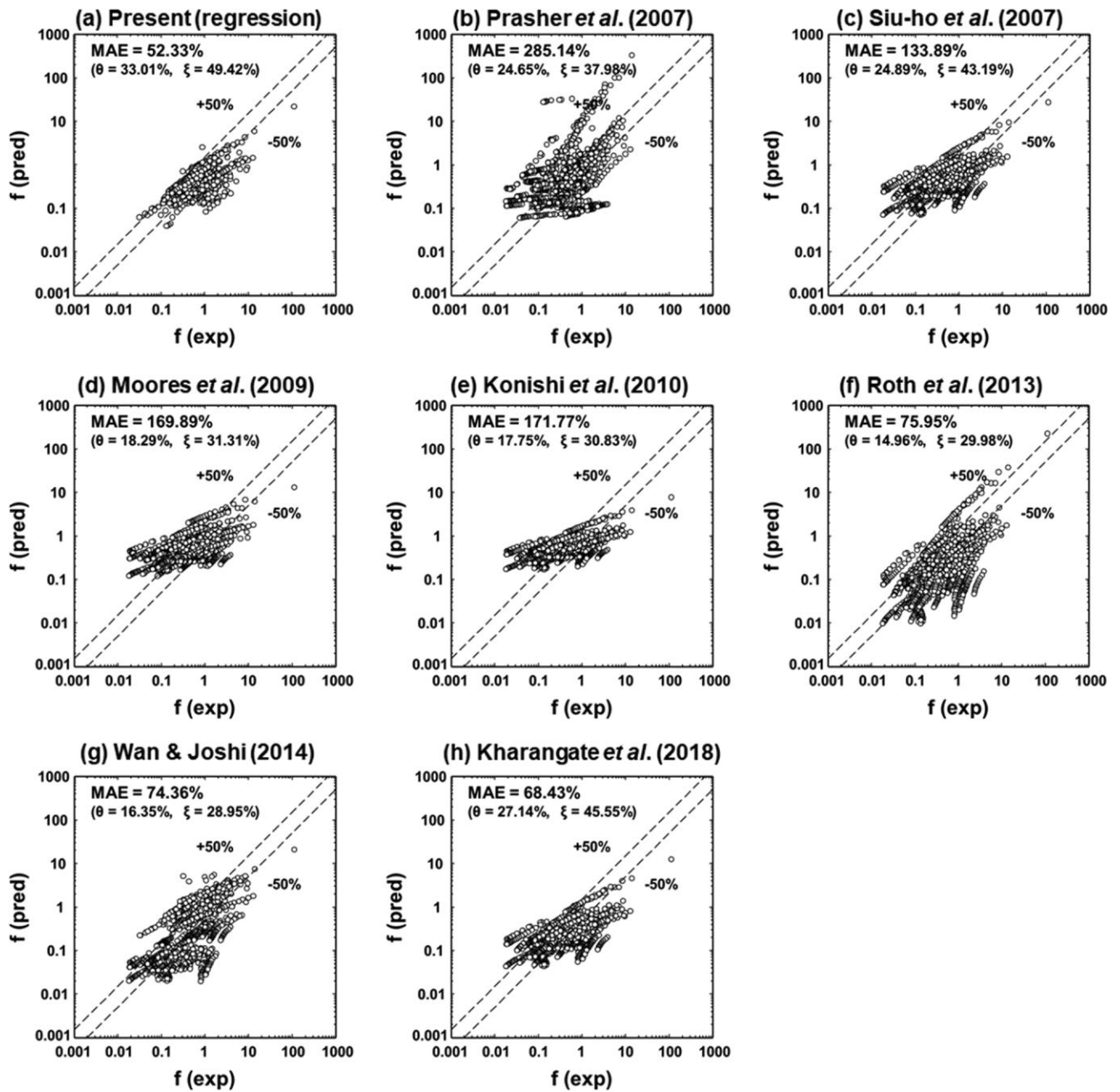
Fig. 7. Comparison of experimentally determined Fanning friction factor with predictions of (a) new regression correlation, (b) Prasher et al. [15], (c) Siu-ho et al. [16], (d) Moore et al. [46], (e) Konishi et al. [17], (f) Roth et al. [47], (g) Wan & Joshi [19], and (h) Kharangate et al. [20].
