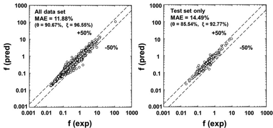
Fig. 11. Comparison of experimentally determined Fanning friction factor with predictions of the MLP model for a) all data set and b) for test data sets.
