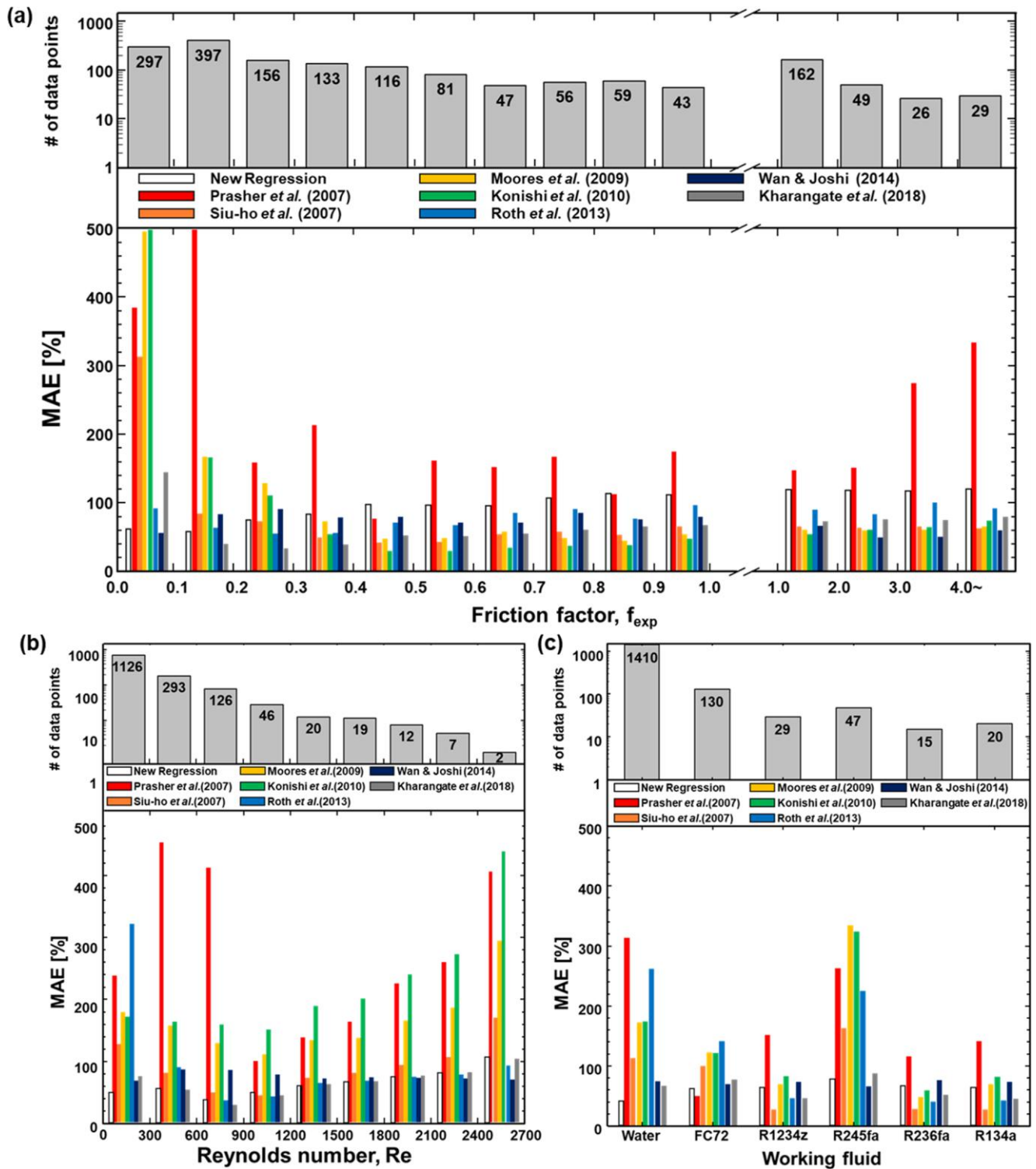
Fig. 9. Distribution of MAE in predictions of present regression correlation and selected relevant correlations relative to (a) friction factor, (b) Reynolds number, and (c) working fluid.
