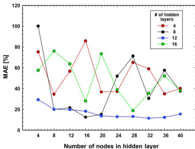
Fig. 6. MLP model predicting accuracies with different combinations of numbers of nodes and hidden layers.
