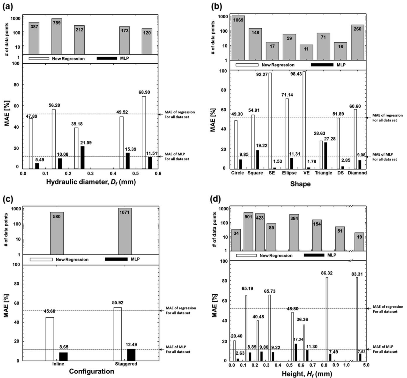
Fig. 13. Distribution of MAE in predictions of MLP for data point relative geometrical conditions: (a) Hydraulic diameter of pin fin, (b) fin shape, (c) fin configuration, and (d) height.
