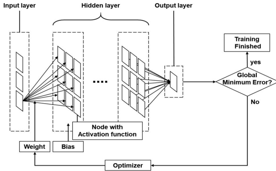
Fig. 5. Architecture of a multilayer perceptron.
