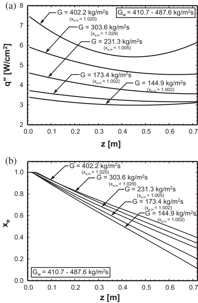
Fig. 9. Variations of (a) heat flux and (b) thermodynamic equilibrium quality along the condensation length for different FC-72 mass velocities.
