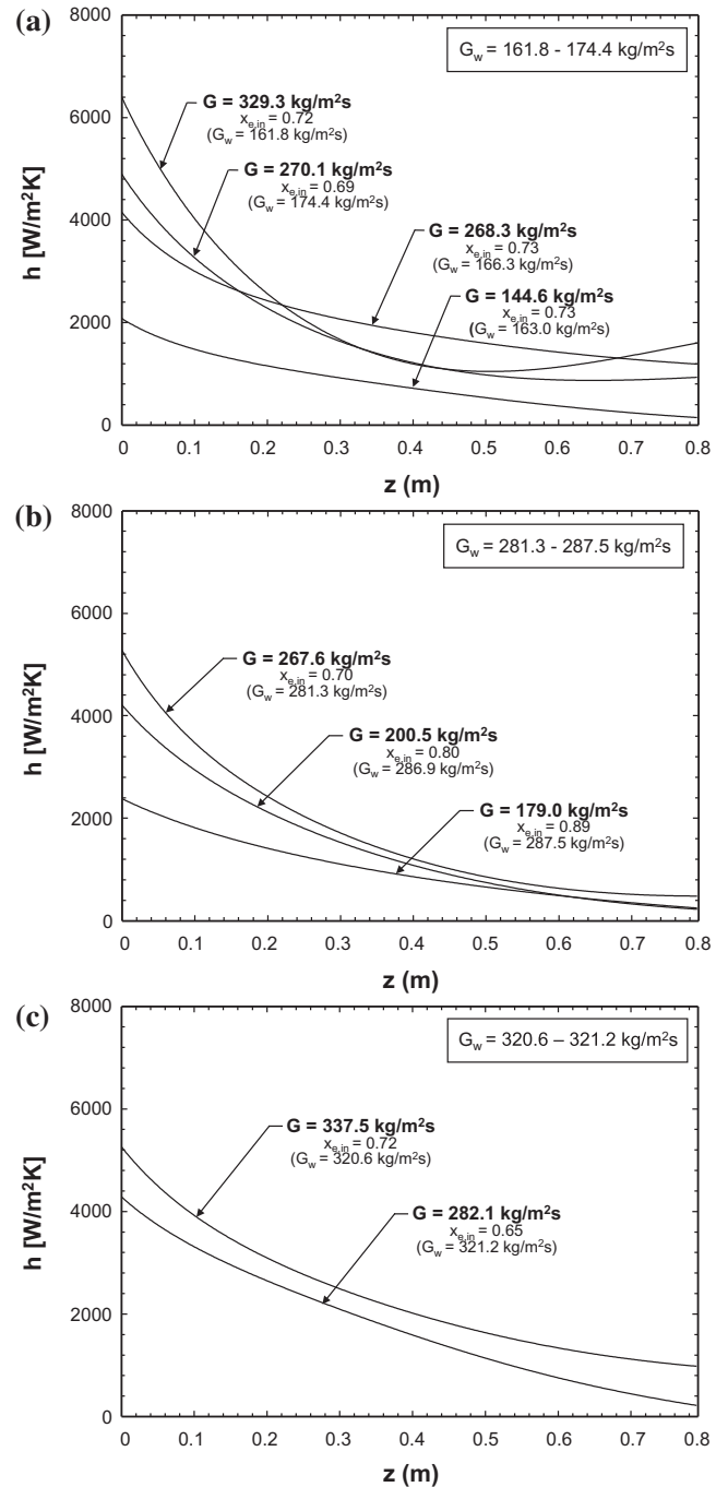
Fig. 9. Variations of experimentally-determined condensation heat transfer coefficient with axial distance for different FC-72 mass velocities and water mass velocities of (a) G_w = 161.8 - 174.4 \text{ kg/m}^2 \text{ s} , (b) G_w = 281.3 - 287.5 \text{ kg/m}^2 \text{ s} and (c) G_w = 320.6 - 321.2 \text{ kg/m}^2 \text{ s} .
