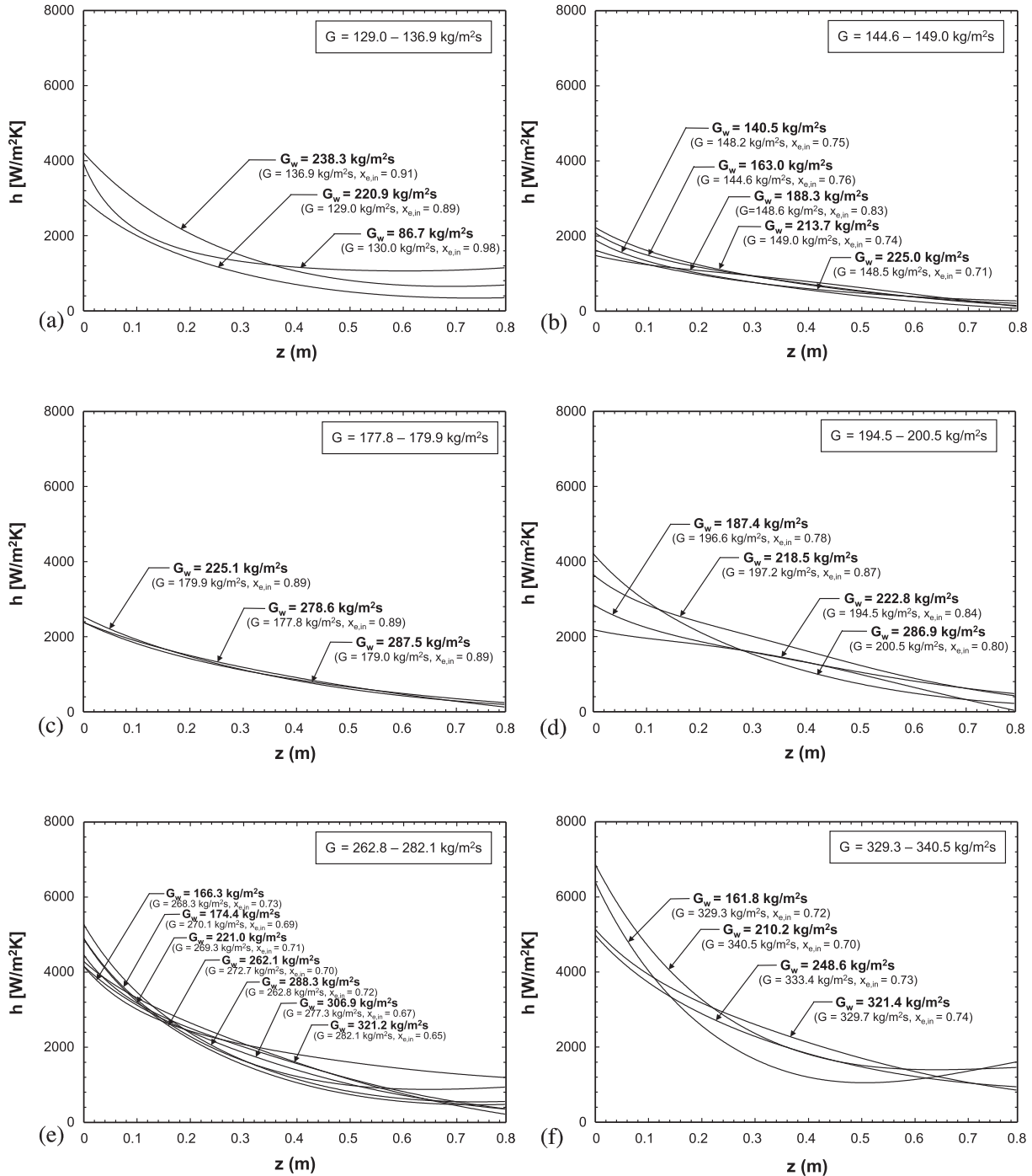
Fig. 10. Variations of experimentally-determined heat transfer coefficient with axial distance for different water mass velocities and FC-72 mass velocities of (a) G = 129.0 - 136.9 \text{ kg/m}^2 \text{ s} , (b) G = 144.6 - 149.0 \text{ kg/m}^2 \text{ s} , (c) G = 177.8 - 179.9 \text{ kg/m}^2 \text{ s} , (d) G = 194.5 - 200.5 \text{ kg/m}^2 \text{ s} , (e) G = 262.8 - 282.1 \text{ kg/m}^2 \text{ s} , and (f) G = 329.3 - 340.5 \text{ kg/m}^2 \text{ s} .
