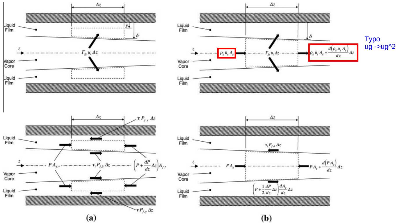
Fig. 11. Momentum and force interactions for (a) liquid film and (b) vapor core control volumes.
