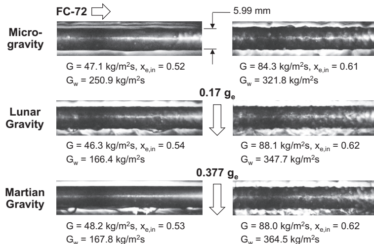
Fig. 5. Comparison of images of condensation film in microgravity, Lunar gravity and Martian gravity for two sets of operating conditions. The images are centered at z = 5.8 \text{ cm} from inlet of condensation length.
