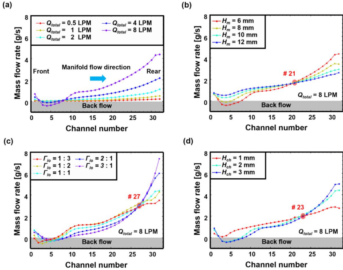
Fig. 5. Mass flow rate across each microchannel at various parameters. (a) Total flow rate, (b) manifold height, (c) ratio of inlet-to-outlet manifold width, and (d) microchannel height. Microchannels near the front section experience lower mass flow rates, including backflows, attributed to the reduced pressure force around the vena contracta. The channels near the rear section experience higher flow rates owing to strong pressure force within the stagnation zone.
