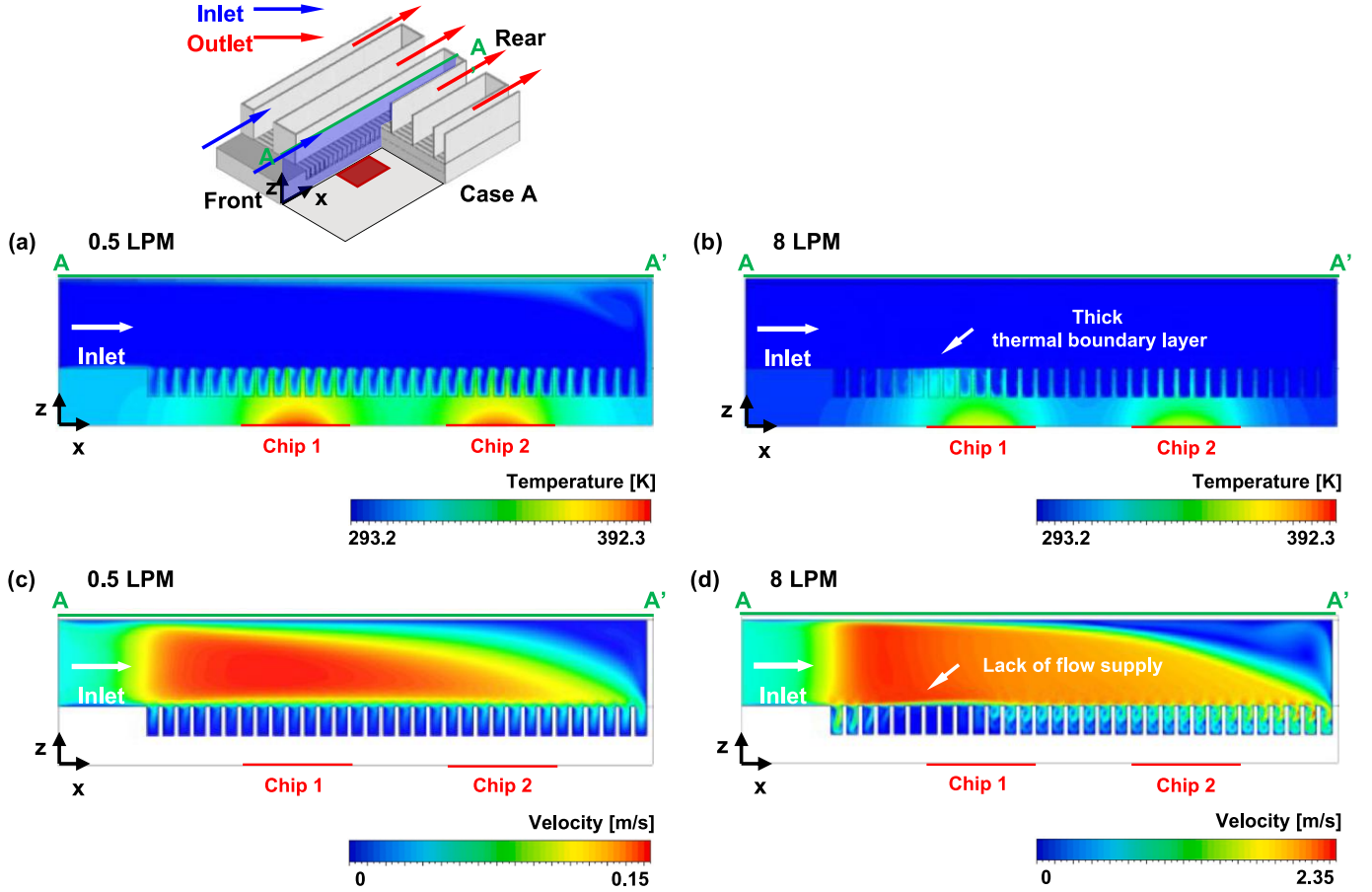
Fig. 11. Temperature and velocity contours of the MMC heat sink at the center of the inlet manifold (Blue Plane): Temperature at (a) 0.5 LPM and (b) 8 LPM, and velocity at (c) 0.5 LPM and (d) 8 LPM. Chip 1 (front section-cooled) exhibits a higher temperature than Chip 2 (rear section-cooled). Therefore, the lack of flow supply around the front section thickens the thermal boundary layer, thereby diminishing the convective heat transfer.
