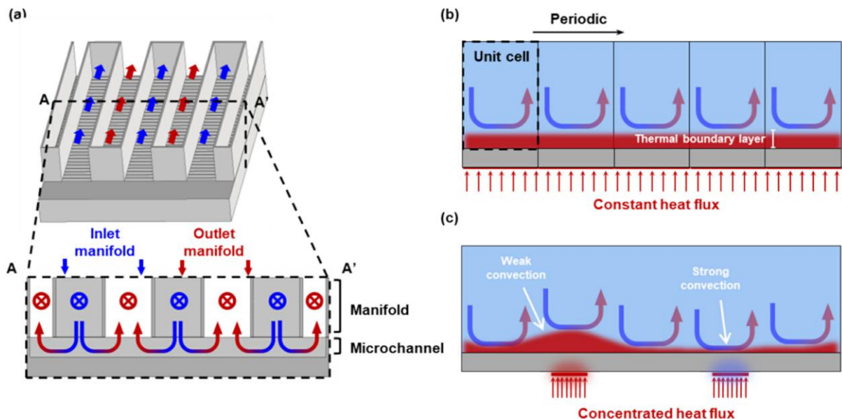
Fig. 1. Schematic illustration of (a) the flow path in an MMC heat sink, (b) the periodically implemented unit cell approach, and (c) the actual non-uniform thermal boundary through the MMC. The working fluid is vertically distributed in the inlet manifold of microchannel and exits from the outlet manifold.
