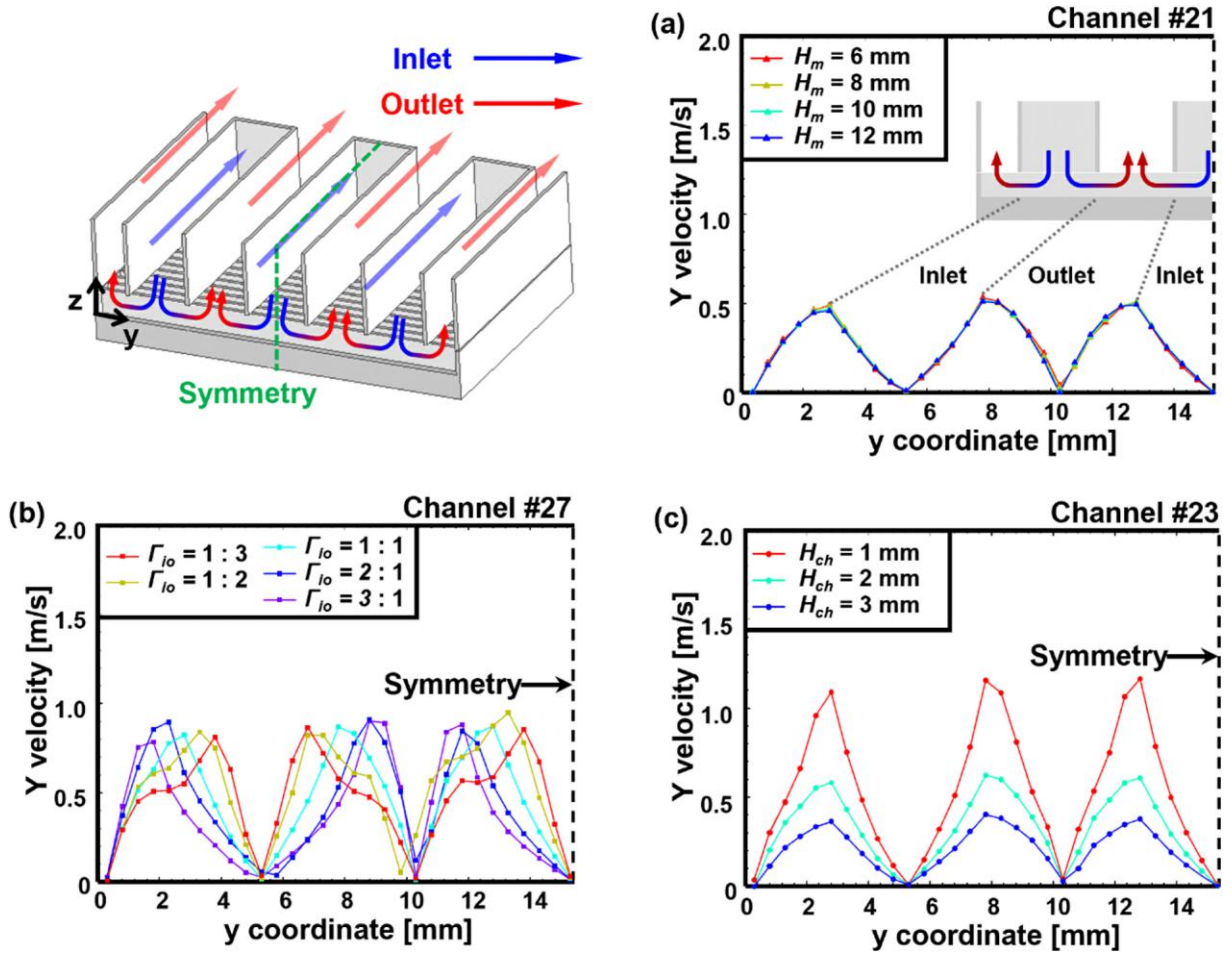
Fig. 8. Comparison of the streamwise (y-direction) velocity distribution within a single microchannel. Total flow rate is fixed at 8 LPM and variations in (a) manifold height, (b) ratio of inlet-to-outlet manifold width, and (c) microchannel height are explored. Stagnation points appear below the manifold center with zero velocity, and streamwise velocity peaks beneath the manifold wall.
