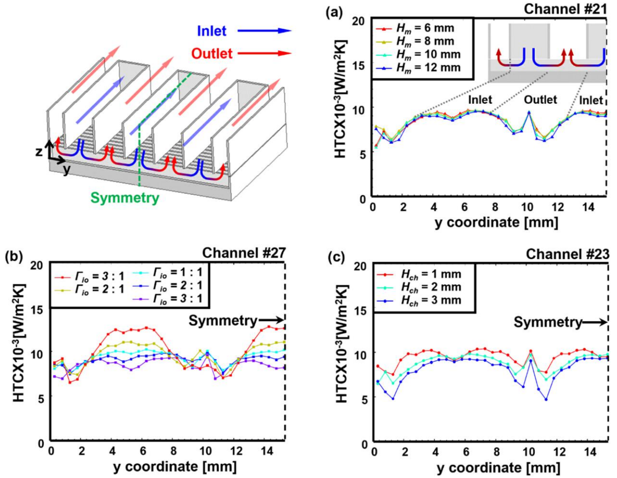
Fig. 10. Heat transfer coefficient distribution within a single microchannel at a total flow rate of 8 LPM. Variations in heat transfer coefficient are compared with (a) manifold height, (b) ratio of inlet-to-outlet manifold width, and (c) microchannel height. A strong relation between streamwise vorticity and velocity is observed, indicating the combined effect of flow stagnation, inertia, and vortex on enhancing the heat transfer.
