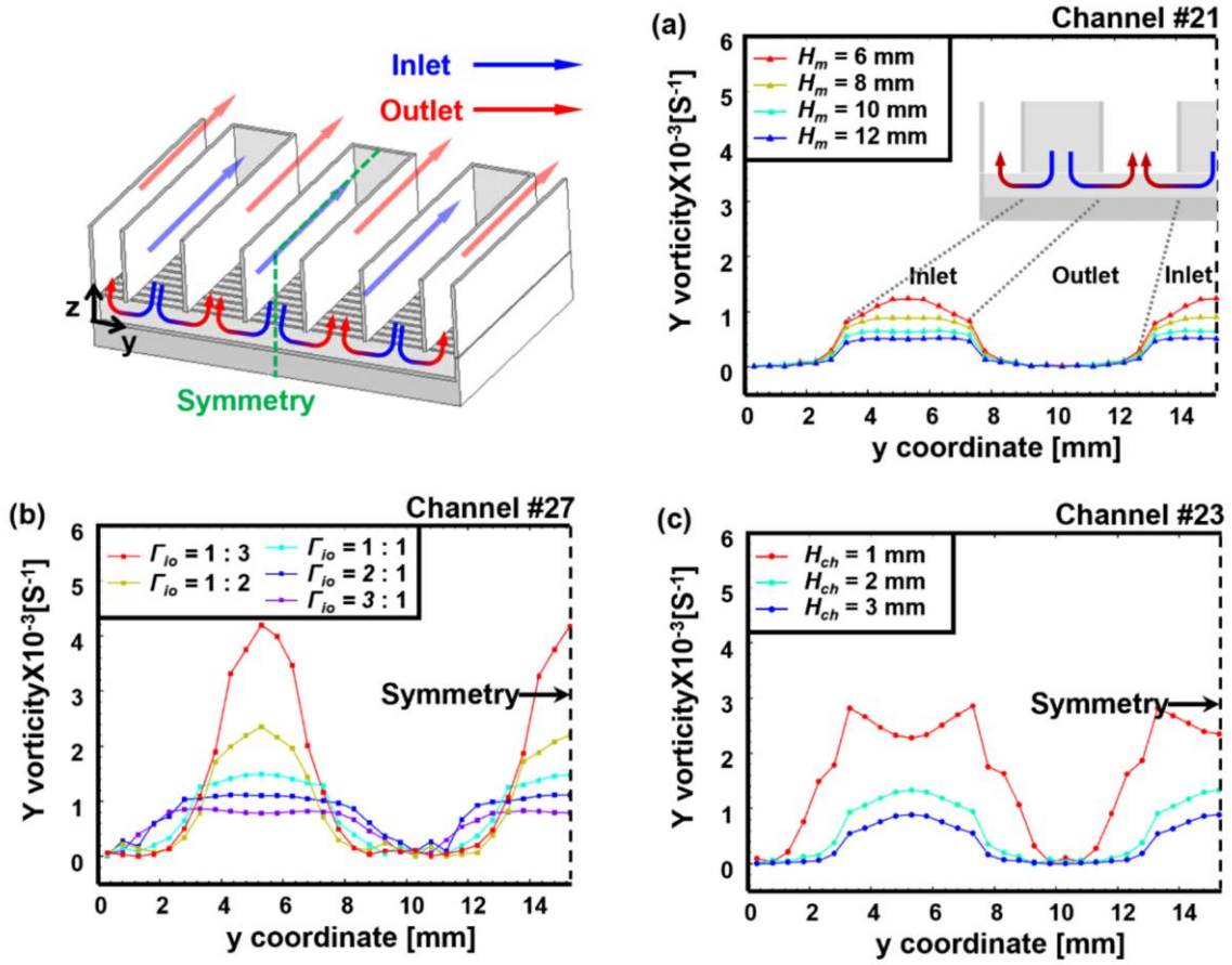
Fig. 9. Comparison of the streamwise ( y -direction) vorticity distribution within a single microchannel. Total flow rate is fixed at 8 LPM and streamwise vorticity distributions are compared by varying (a) manifold height, (b) ratio of inlet-to-outlet manifold width, and (c) microchannel height. Streamwise vortex, which appears below the inlet manifold and disappears beneath the outlet manifold, intensifies with decreasing inlet manifold width and microchannel height.
