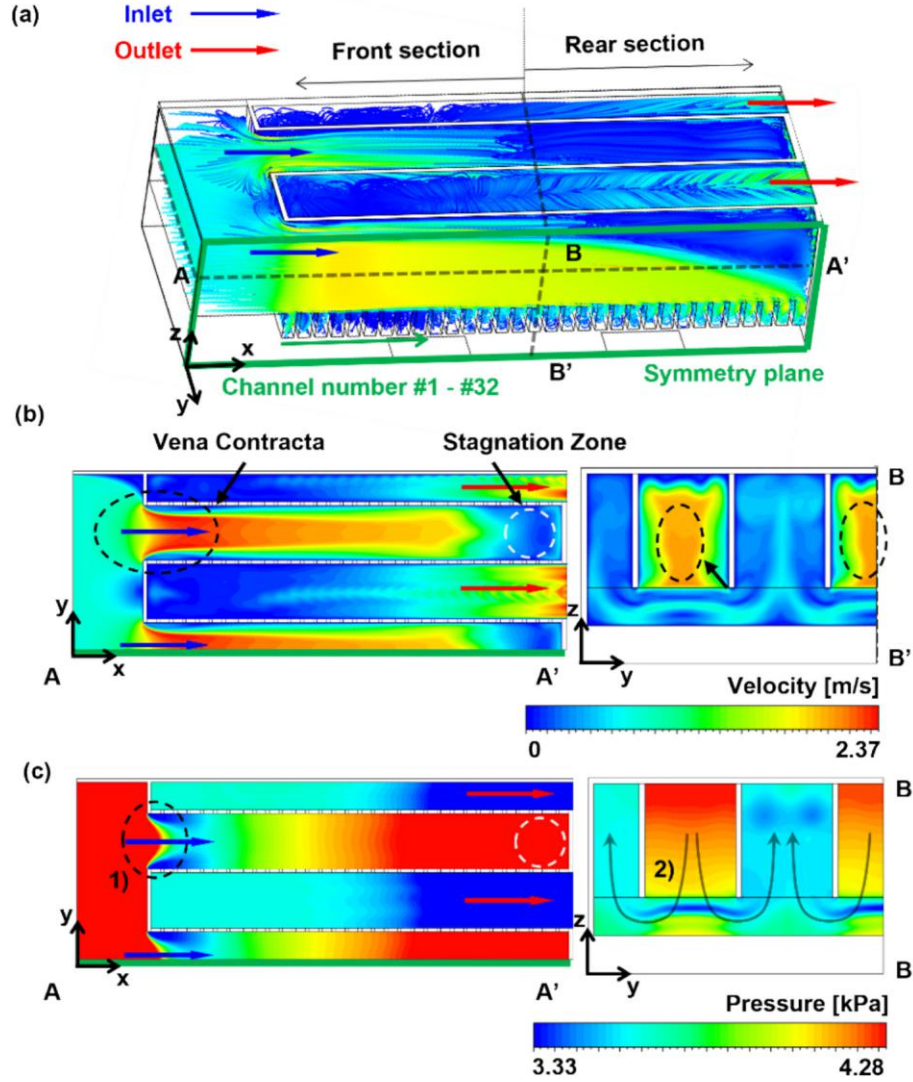
Fig. 4. Flow morphology within the full-scale MMC heat sink (a) Streamlines on a half-domain with contours of the velocity magnitude. (b) Velocity and (c) pressure contours at the center plane in Case A under a flow rate of 8 LPM. Distinct flow phenomena, including vena contracta and stagnation zones, are depicted. These regions influence the static pressure distribution and expose extra pressure losses in the MMC heat sink.
