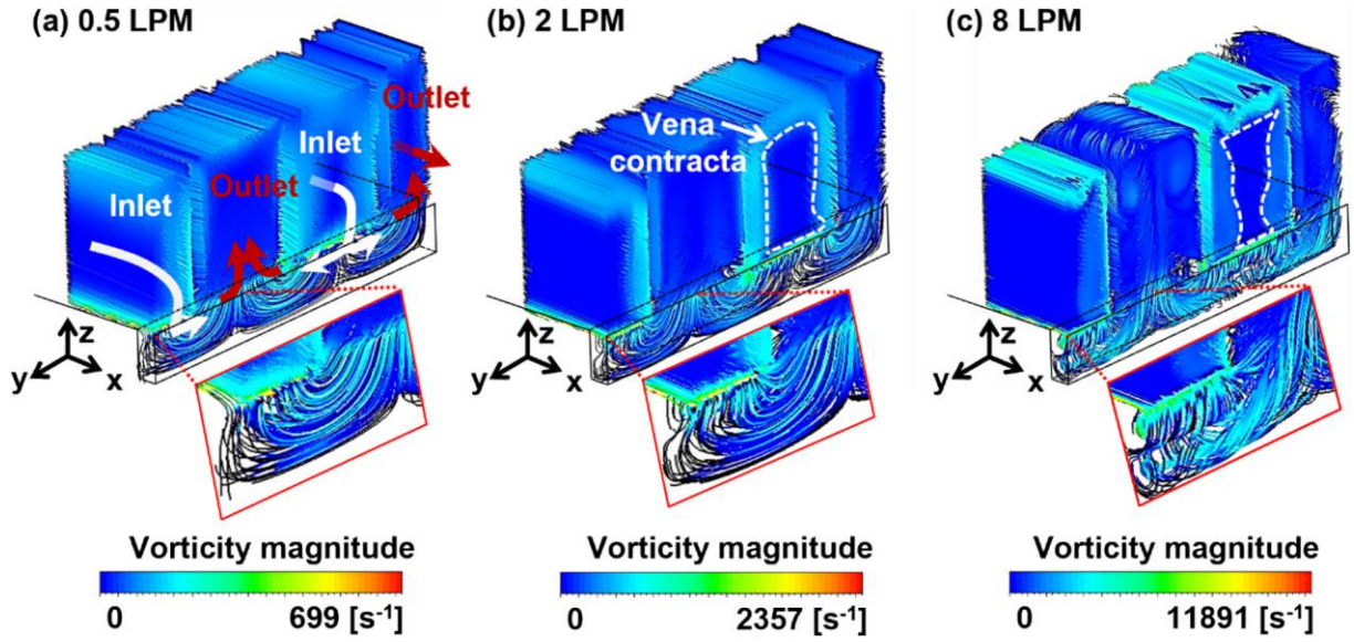
Fig. 7. Streamlines at the center of the MMC heat sink with vorticity magnitude contours. Vortex formation in the microchannel flow is depicted at the following flow rates: (a) 0.5 LPM, (b) 2 LPM, and (c) 8 LPM. Lower flow rates exhibit a smooth profile, whereas higher flow rates induce persistent streamwise vortex along the microchannel.
