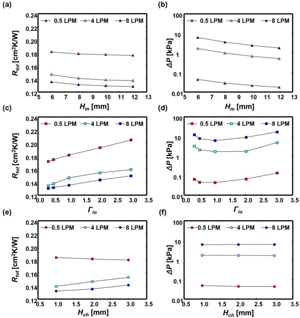
Fig. 12. Total thermal resistance and pressure drop in various MMC heat sinks. Variations in (a, b) manifold height, (c, d) ratio of inlet-to-outlet manifold width, and (e, f) microchannel height. Comparison at the flow rates of 0.5, 4, and 8 LPM reveals distinct trends. Independent of the total flow rate, decreased manifold width reduces thermal resistance and increased manifold height enhances pressure drop and thermal resistance. Decreased microchannel height provides a lower thermal resistance at high rate (4 and 8 LPM), whereas it results in higher thermal resistance at a low flow rate (0.5 LPM).
