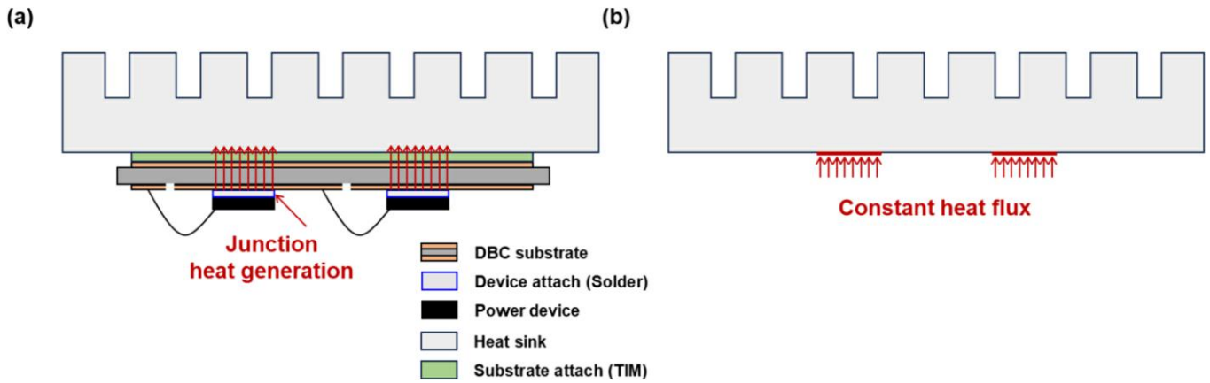
Fig. 2. Schematic illustration of conventional 2-in-1 SiC power module cooling architecture packaging layers with heat generation at the device junction, and (b) a simplified model with constant heat flux conditions.
