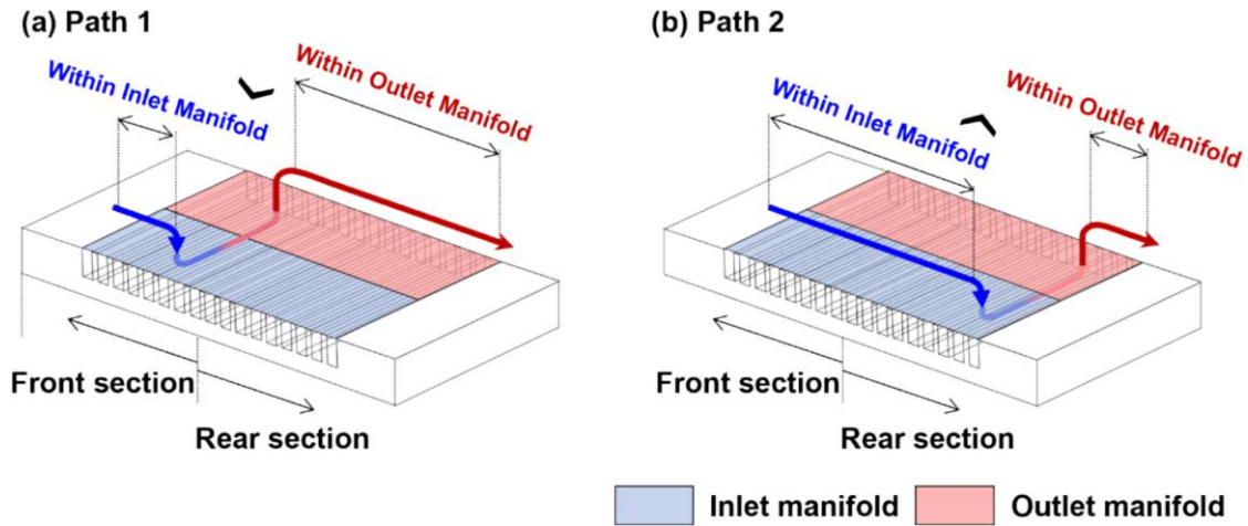
Fig. 6. Schematic of the two flow paths within the MMC heat sink. (a) Path 1 through channels near the front section and (b) Path 2 through channels near the rear section. Paths 1 and 2 have a longer distance of travel within the outlet and inlet manifolds, respectively.
